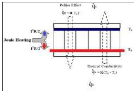
Figure 1. Heat transfer in thermoelectric
