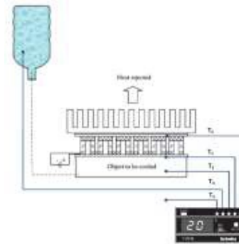
Figure2. Single Thermoelectric Testing Installation
