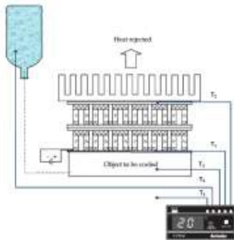
Figure 3. Double Thermoelectric Testing Installation
