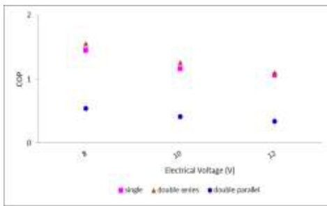
Figure 6. Graphs of the relationship of voltage applied to the COP on 360 minutes
