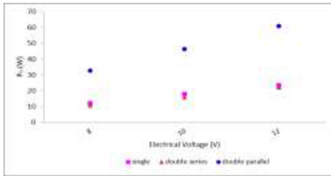
Figure 5. Graph of electricity voltage to the electrical power supplied with the circuit variation on 360 minutes.
